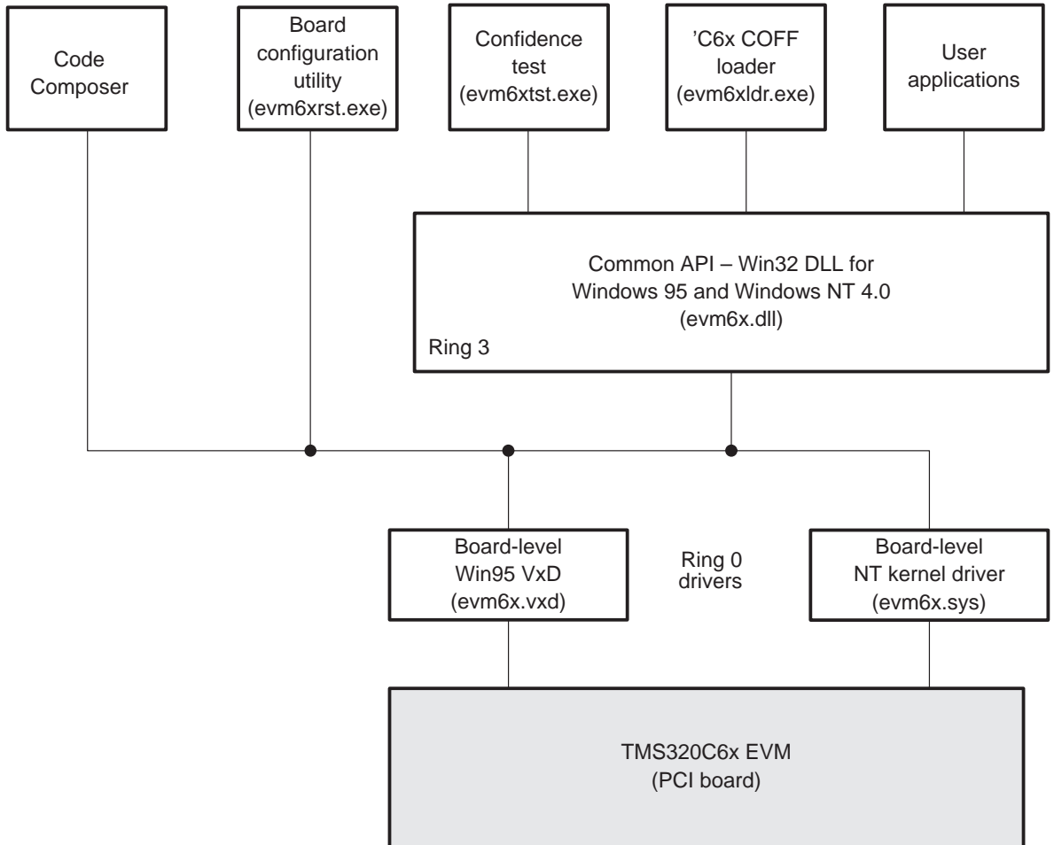
Figure 1–4. TMS320C6x EVM Host Support Software Block Diagram
